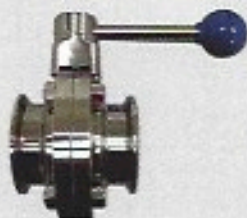
140123 Valve, 1-1/2", 316SS, Sanitary Butterfly, Tri Clamp, IN LINE CLOSED handle
